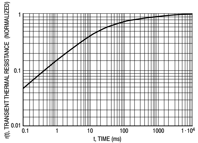
Figure 4. Thermal Response
